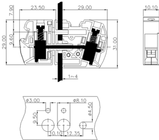
钻孔图 For a drilling diagram
